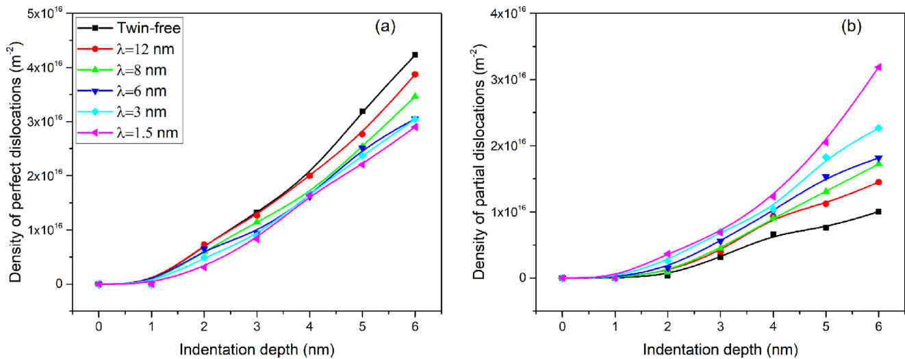
Fig. 4. Evolution of density of (a) perfect and (b) partial dislocations with indentation depth in the nanotwinned single crystalline substrates.
