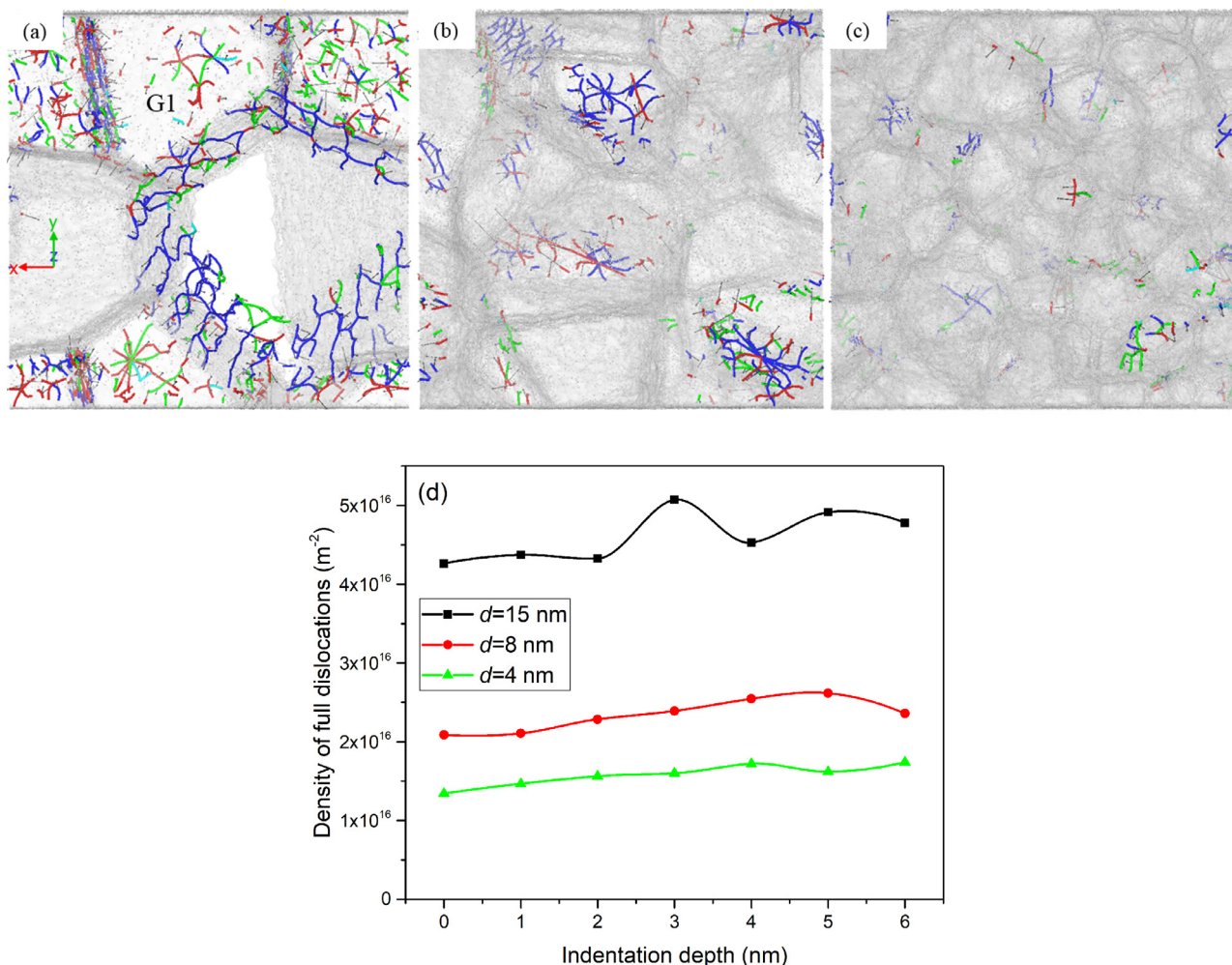
Fig. 8. Pre-existing dislocations at the GBs of the twin-free nanocrystalline substrates with (a) d = 15 nm, (b) d = 8 nm, (c) d = 4 nm; (d) Density of full dislocations as a function of the indentation depth.
