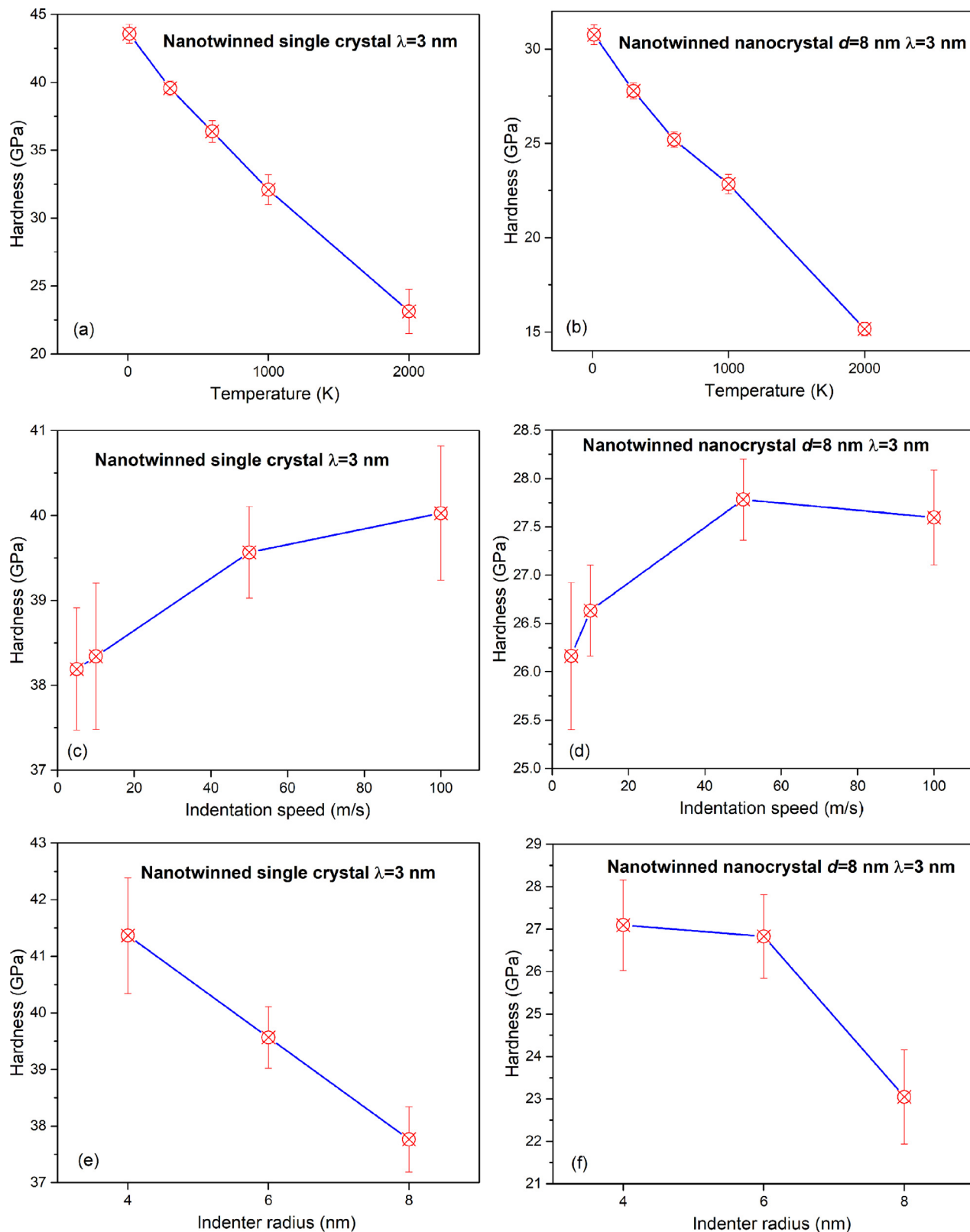
Fig. 18. Effect of (a-b) temperature, (c-d) indentation speed, and (e-f) indenter size on the hardness of nanotwinned single crystalline and nanocrystalline samples.
