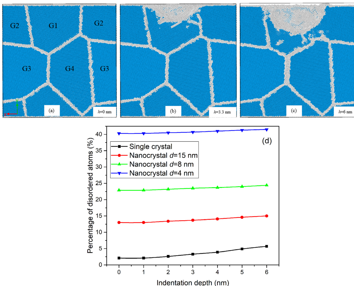
Fig. 10. (a–c) Crystalline intragranular (in blue color) and disordered intergranular (in white color) phases in the nanocrystalline 3C-SiC with d = 15 nm, (b–c) GB and triple junction migration between G1 and G2, (d) Percentage of disordered atoms as a function of indentation depth. (For interpretation of the references to colour in this figure legend, the reader is referred to the web version of this article.)
