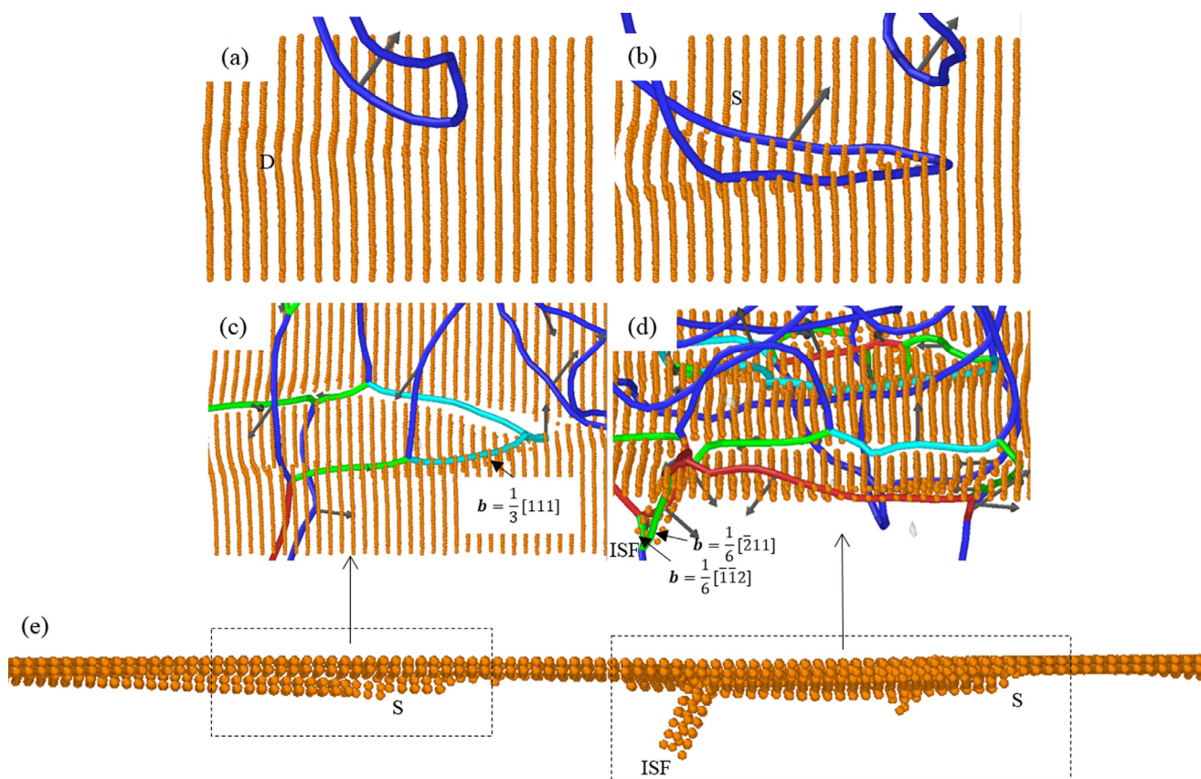
Fig. 6. (a–d) Detailed atomic structures of CTB in the nanotwinned 3C-SiC substrate with \lambda=12 nm, (e) Side view of the CTB showing the formation of steps and nucleation of a Shockley partials accompanied by a stacking fault from the defective CTB. D, distortion of the CTB due to the incoming dislocations; S, slip; ISF, intrinsic stacking fault. (For interpretation of the references to colour in this figure legend, the reader is referred to the web version of this article.)
