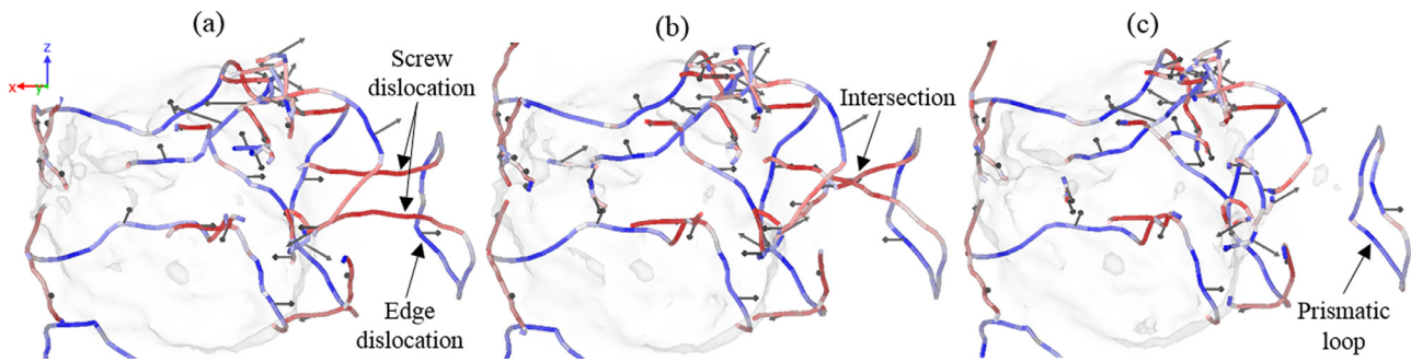
Fig. 3. Formation of prismatic loops as a result of “Lasso”-like mechanism via intersection and annihilation of screw dislocations at h \sim 1.8 nm. Dislocations are colored based on the dislocation character, with the screw components in red and edge components in blue. (For interpretation of the references to colour in this figure legend, the reader is referred to the web version of this article.)
