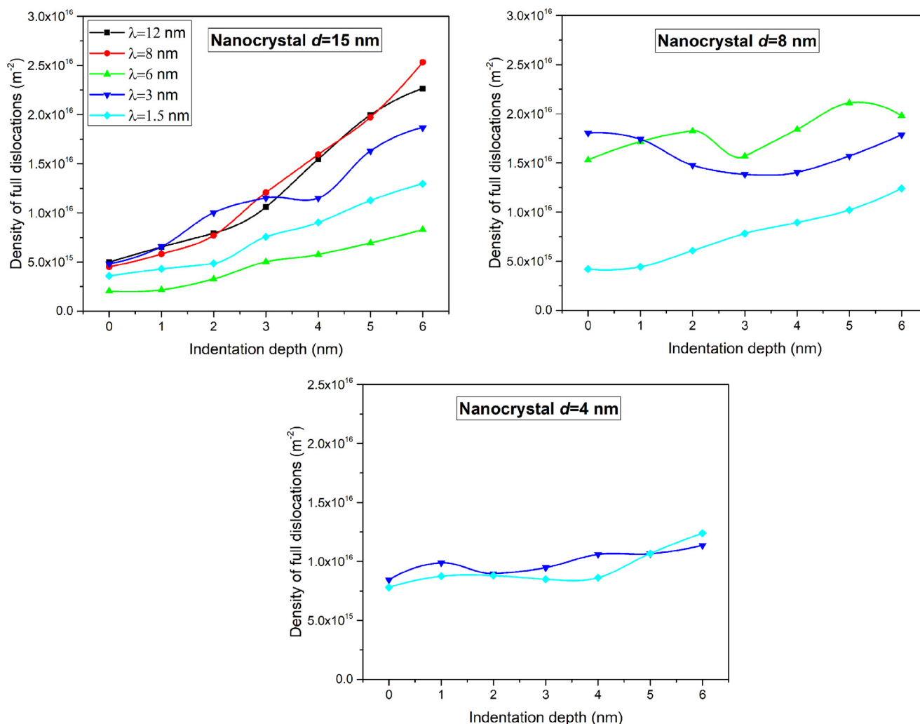
Fig. 12. Density evolution of full dislocations with indentation depth for the nanotwinned nanocrystalline 3C-SiC.
