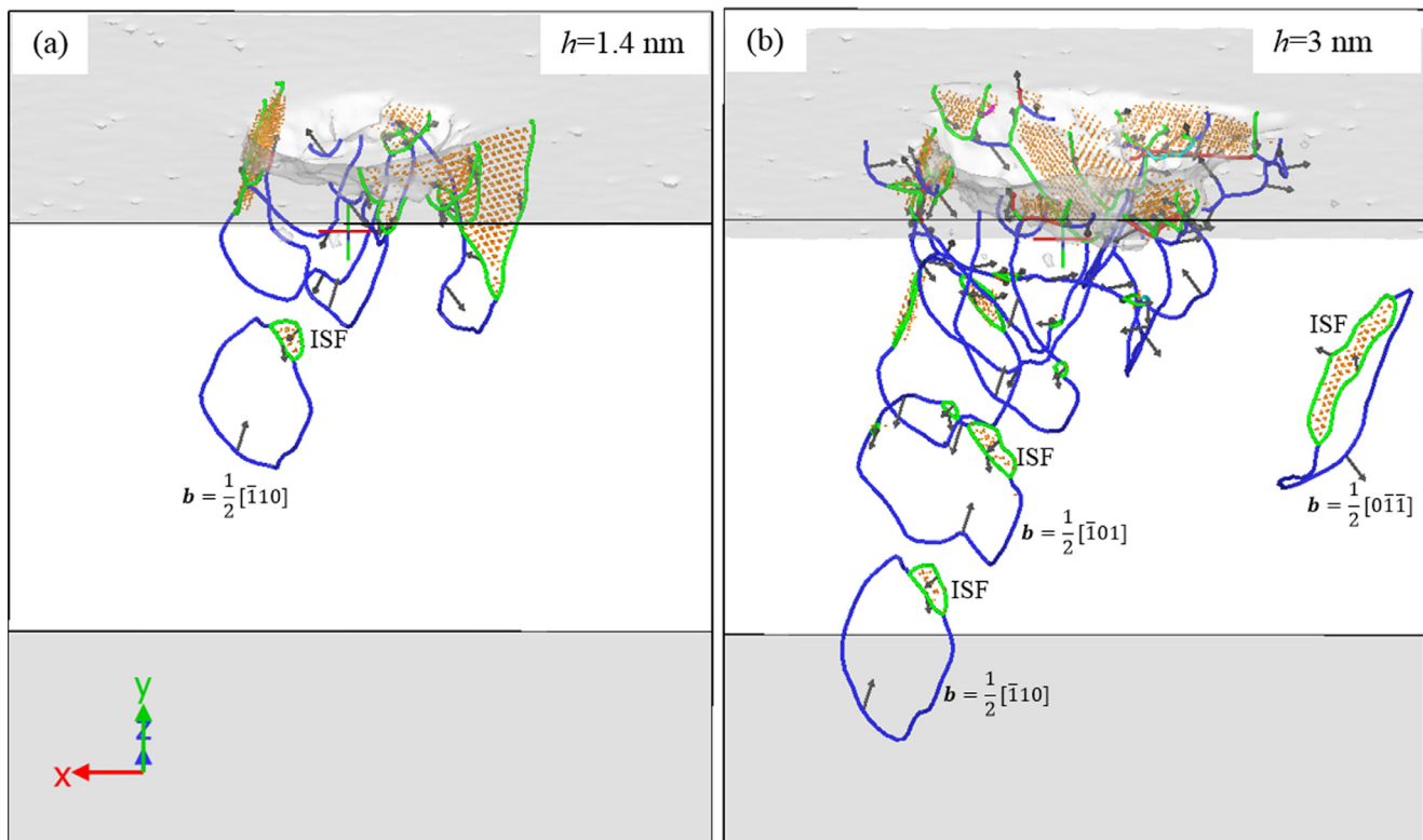
Fig. 15. Snapshots showing the formation of ISFs, surrounded by Shockley partials, within the prismatic loops in the twin-free single crystal at T = 1000 K.
