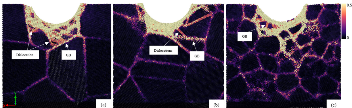
Fig. 11. Local shear strain distribution in the XY plane in the twin-free nanocrystalline substrates with (a) d = 15 nm, (b) d = 8 nm, and (c) d = 4 nm, respectively, at h = 5 nm.
