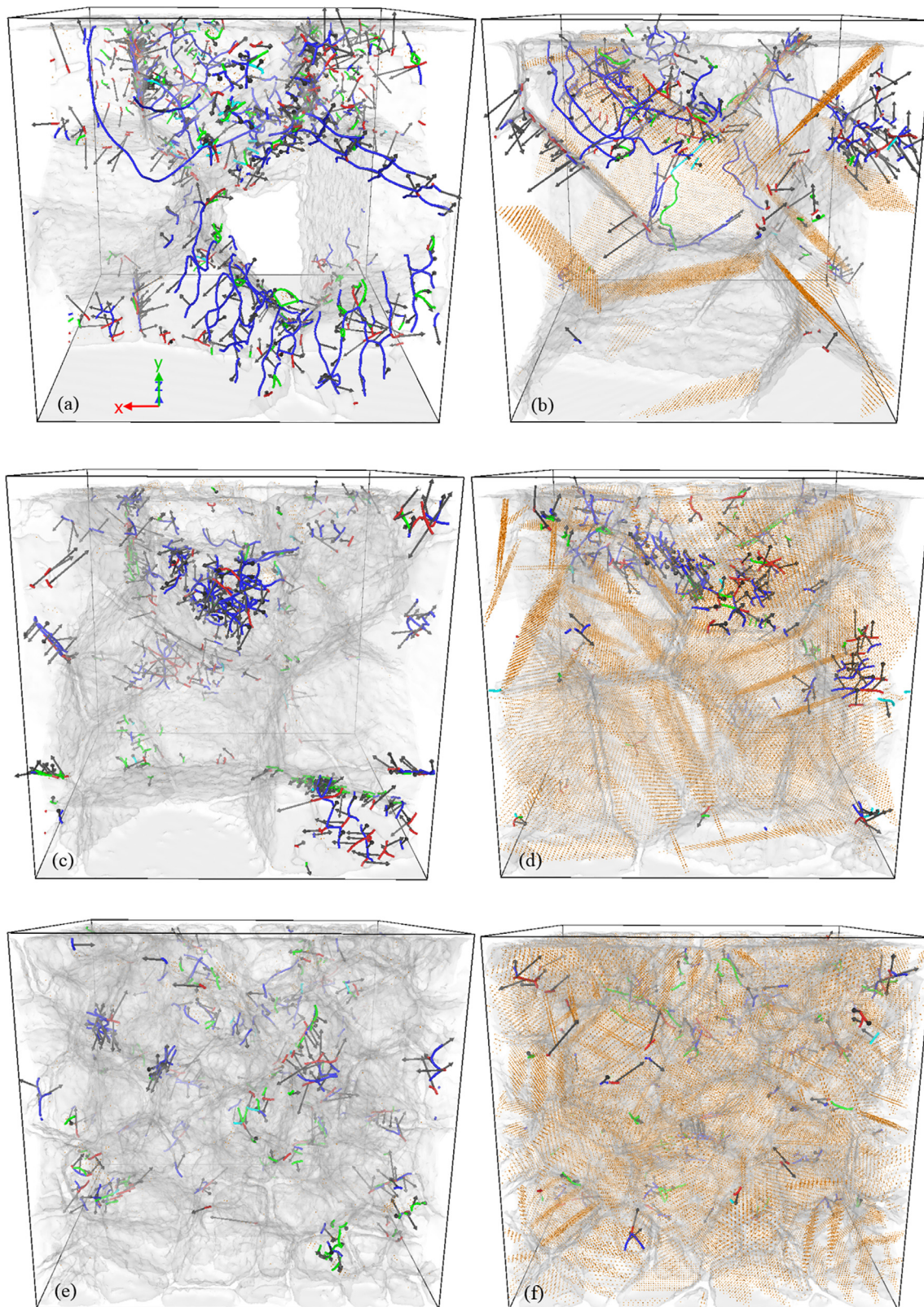
Fig. 7. Snapshots showing the dislocation network inside the nanocrystalline 3C-SiC at h = 6 nm, for some representative cases (a-b) Twin-free and nanotwinned ( \lambda = 8 nm) samples with d = 15 nm, (c-d) Twin-free and nanotwinned ( \lambda = 3 nm) samples with d = 8 nm, (e-f) Twin-free and nanotwinned ( \lambda = 1.5 nm) samples with d = 4 nm. (For interpretation of the references to colour in this figure legend, the reader is referred to the web version of this article.)
