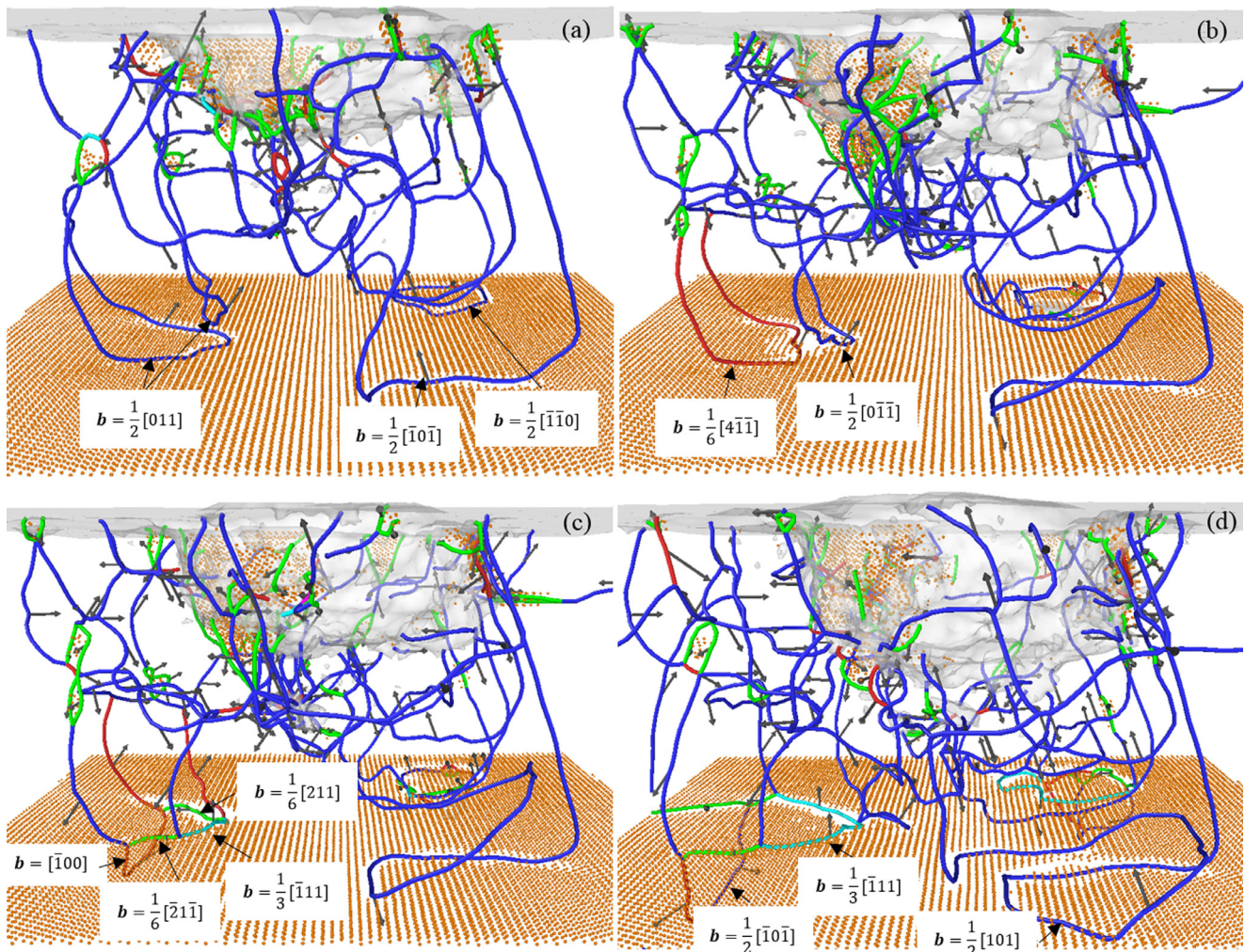
Fig. 5. Dislocation-CTB interaction in the nanotwinned 3C-SiC substrate with \lambda=12 nm. (For interpretation of the references to colour in this figure legend, the reader is referred to the web version of this article.)
