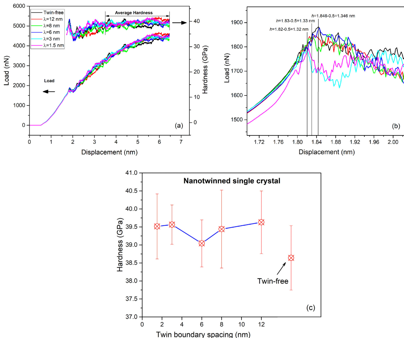
Fig. 16. (a) Indentation load-displacement and hardness-displacement curves of the twin-free and nanotwinned single crystal samples, (b) Zoomed view of the load-displacement where pop-in occurs, (c) variation of average indentation hardness with \lambda . The error bars represent standard deviation.
