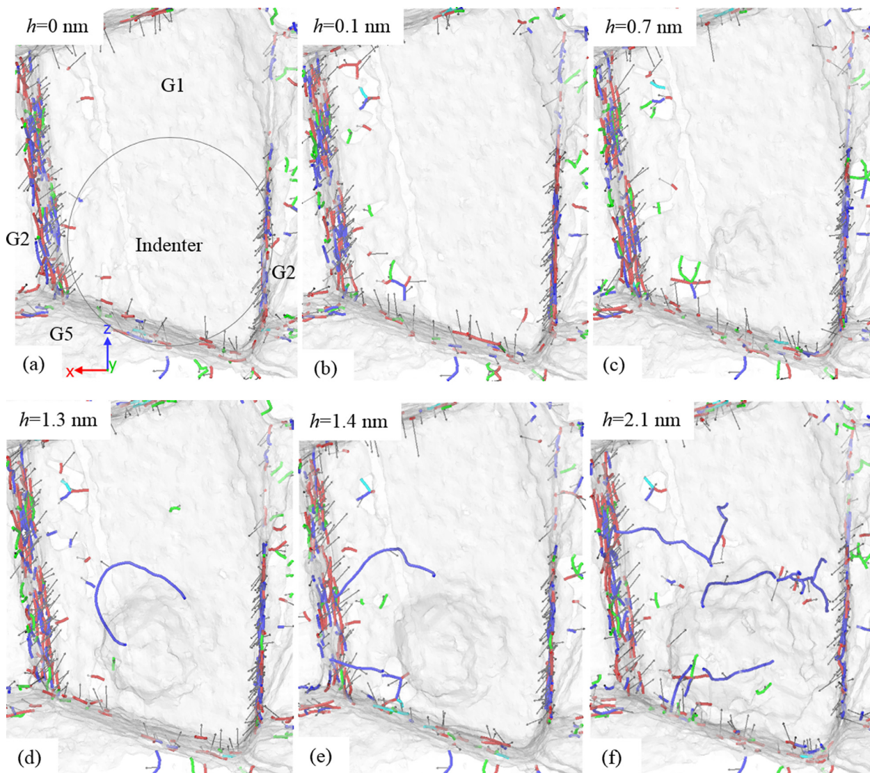
Fig. 9. Incipient of dislocation activity in the grain lying directly under the indenter (G1) for the nanocrystalline substrate with d = 15 nm.
