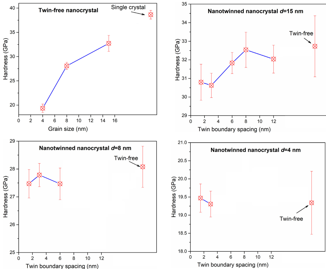
Fig. 17. Variation of hardness of twin-free and nanotwinned nanocrystalline samples with grain size and CTB spacing.
