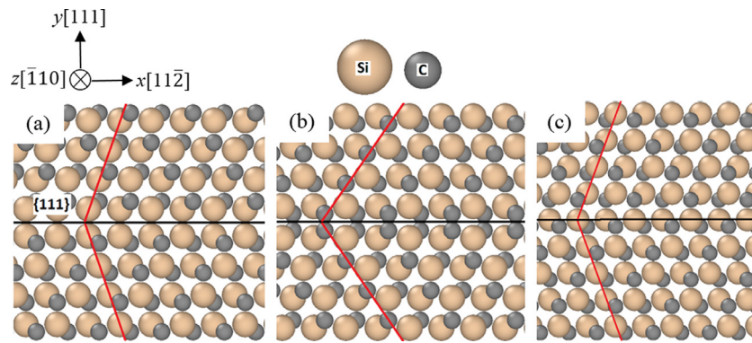
Fig. 1. Schematic illustrations of atomic arrangements of \{111\} \Sigma 3 CTBs in 3C-SiC: (a) Symmetric Si-Si bonded twin with complete mirror lattices on both sides of the CTB; (b) Symmetric C-C bonded twin with complete mirror lattices on both sides of the CTB; (c) Asymmetric Si-C bonded twin without mirror symmetry.
