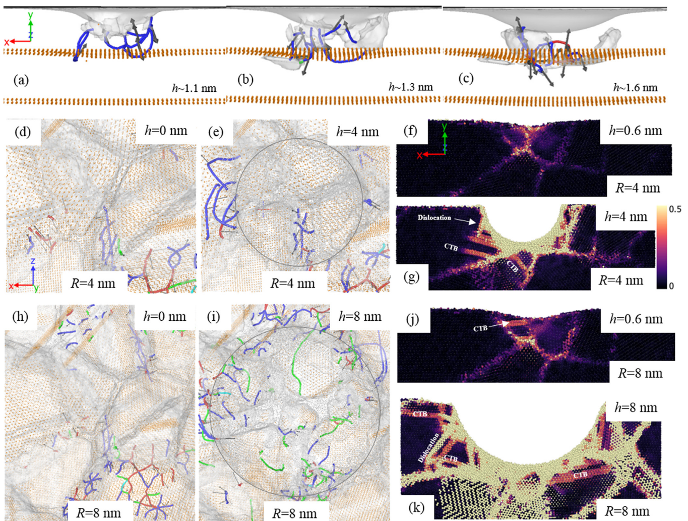
Fig. 14. Defect structure of nanotwinned single crystal with \lambda = 3 nm under the indenter at the initial stage of plasticity for the indenter sizes of (a) R = 4 nm, (b) R = 6 nm, (c) R = 8 nm; (d–i) and (f–k) Defect structure and von Mises shear strain distribution of the nanotwinned nanocrystal with d = 8 nm and \lambda = 3 nm in the XY plane, respectively, with different R . (For interpretation of the references to colour in this figure legend, the reader is referred to the web version of this article.)
