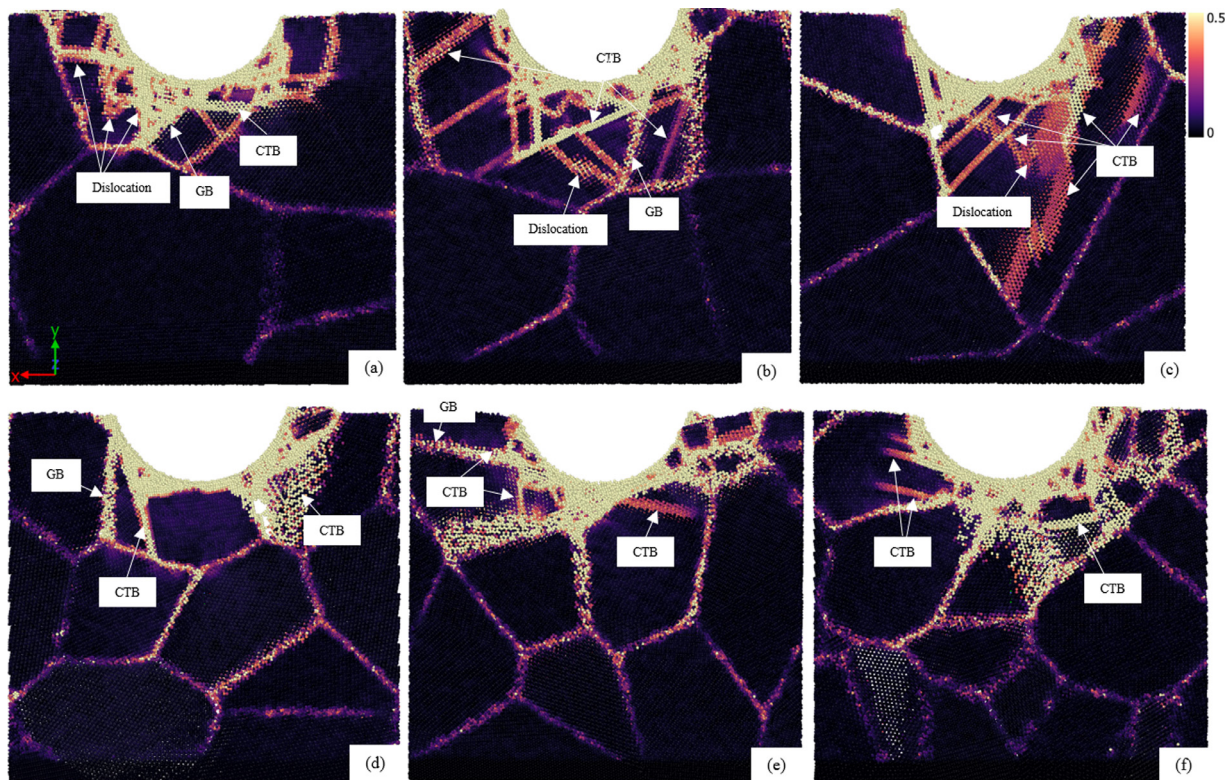
Fig. 13. The microstructures of the nanotwinned nanocrystalline substrates in the XY plane under indentation at h = 5 nm. Atoms are colored according to their local shear strain, (a) d = 15 nm, \lambda = 12 nm, (b) d = 15 nm, \lambda = 6 nm, (c) d = 15 nm, \lambda = 1.5 nm, (d) d = 8 nm, \lambda = 6 nm, (e) d = 8 nm, \lambda = 1.5 nm, (f) d = 4 nm, \lambda = 1.5 nm. A one-to-one comparison with the DXA snapshots is carried out to distinguish lattice dislocations from CTBs, both of which are in ivory color.
