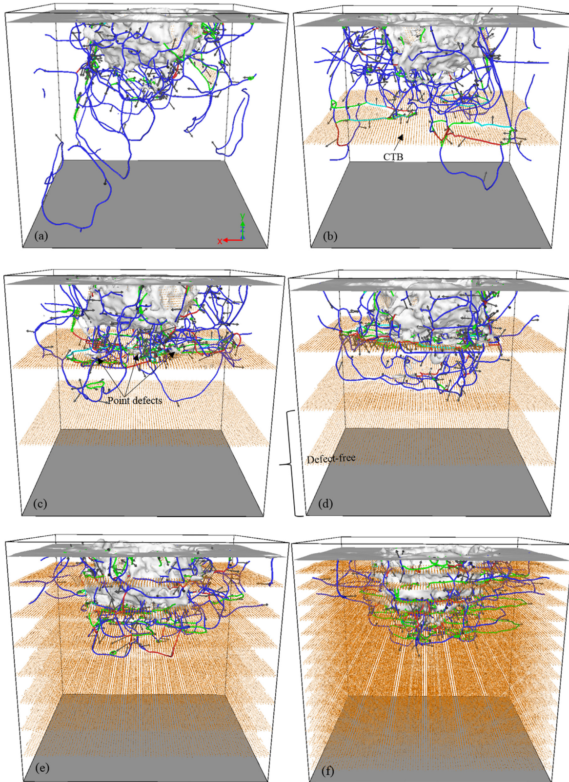
Fig. 2. Overall defect network of indented single crystalline 3C-SiC substrate at h = 6 nm. (a) Twin-free, (b) \lambda = 12 nm, (c) \lambda = 8 nm, (d) \lambda = 6 nm, (e) \lambda = 3 nm, (f) \lambda = 1.5 nm. Dislocation lines are colored according to their Burgers vector i.e. blue, green, aqua, and red lines, respectively, represent the perfect, Shockley partial, Frank partial, and other partial dislocations. Black arrows designate directions of \mathbf{b} . (For interpretation of the references to colour in this figure legend, the reader is referred to the web version of this article.)
